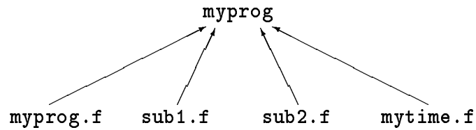
Figure 3: Derivation of Multi-Modular myprog.
