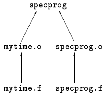
Figure 5: Derivation of specprog .
