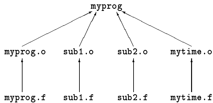
Figure 4: Alternate Derivation of Multi-Modular myprog.
