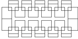
Figure 6: An example with performance ratio 4/3 .
