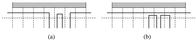
Figure 3: By performing local modifications, an optimal cycle cover can be assumed to cover each piece of the boundary in one connected link.
